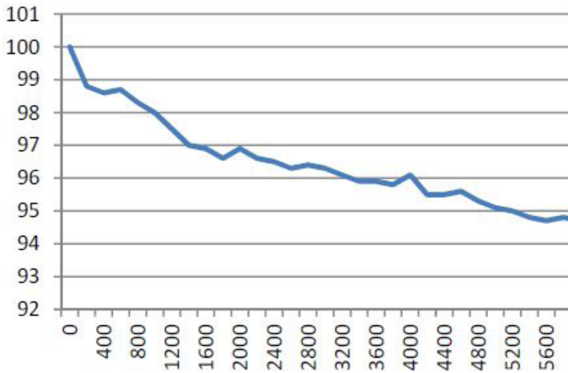
Lumen maintenance
